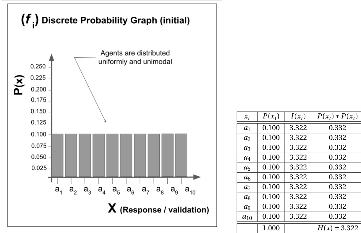
Figure 2: Discrete probability graph at initial state f^i
