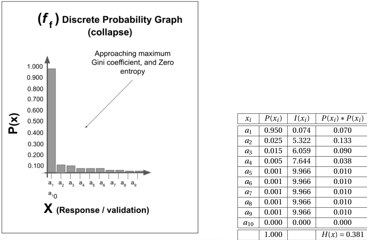
Figure 6: As the Gini coefficient of a power-law distribution increases to maximum, the entropy approaches zero.
