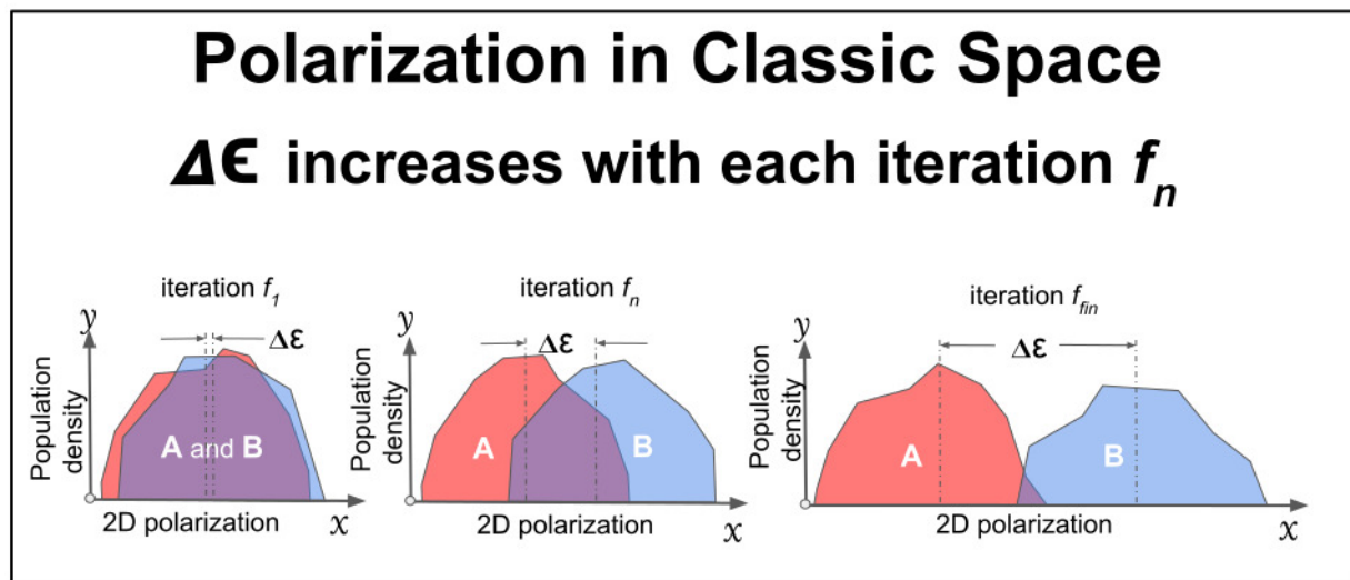
Figure 7: Polarization tends to emerges in the natural world (classic space) over iterations f_n
