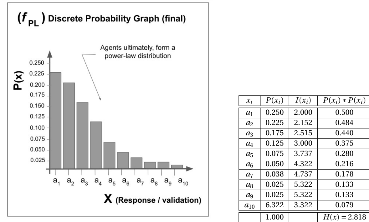
Figure 5: Discrete probability graph transitioning to a power-law distribution
