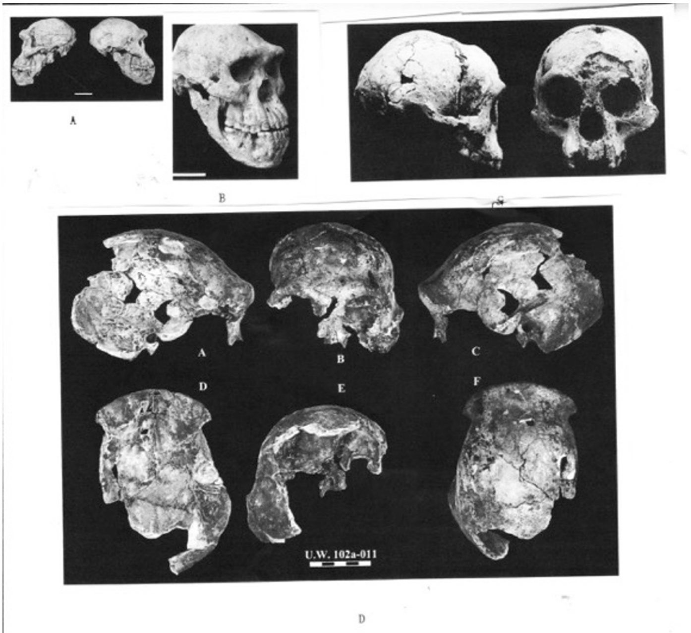
Figure 1. Some Small-Bodied Hominin Crania: A. and B. Skull 5 from Dmanisi 1.8 my; Rightmire [38]; C. LB1 Homo floresiensis , Baab, et al. [36]; D. Homo naledi , Berger, et al. [39].
