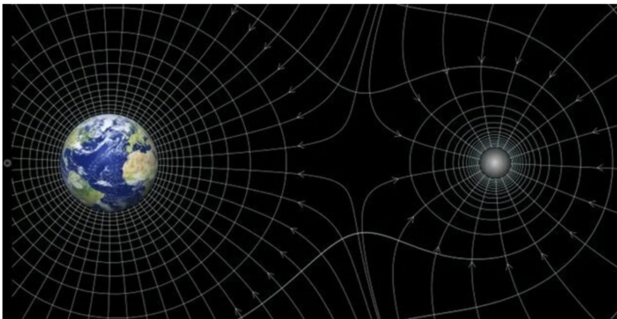
Fig. 1. Lagrangian model
