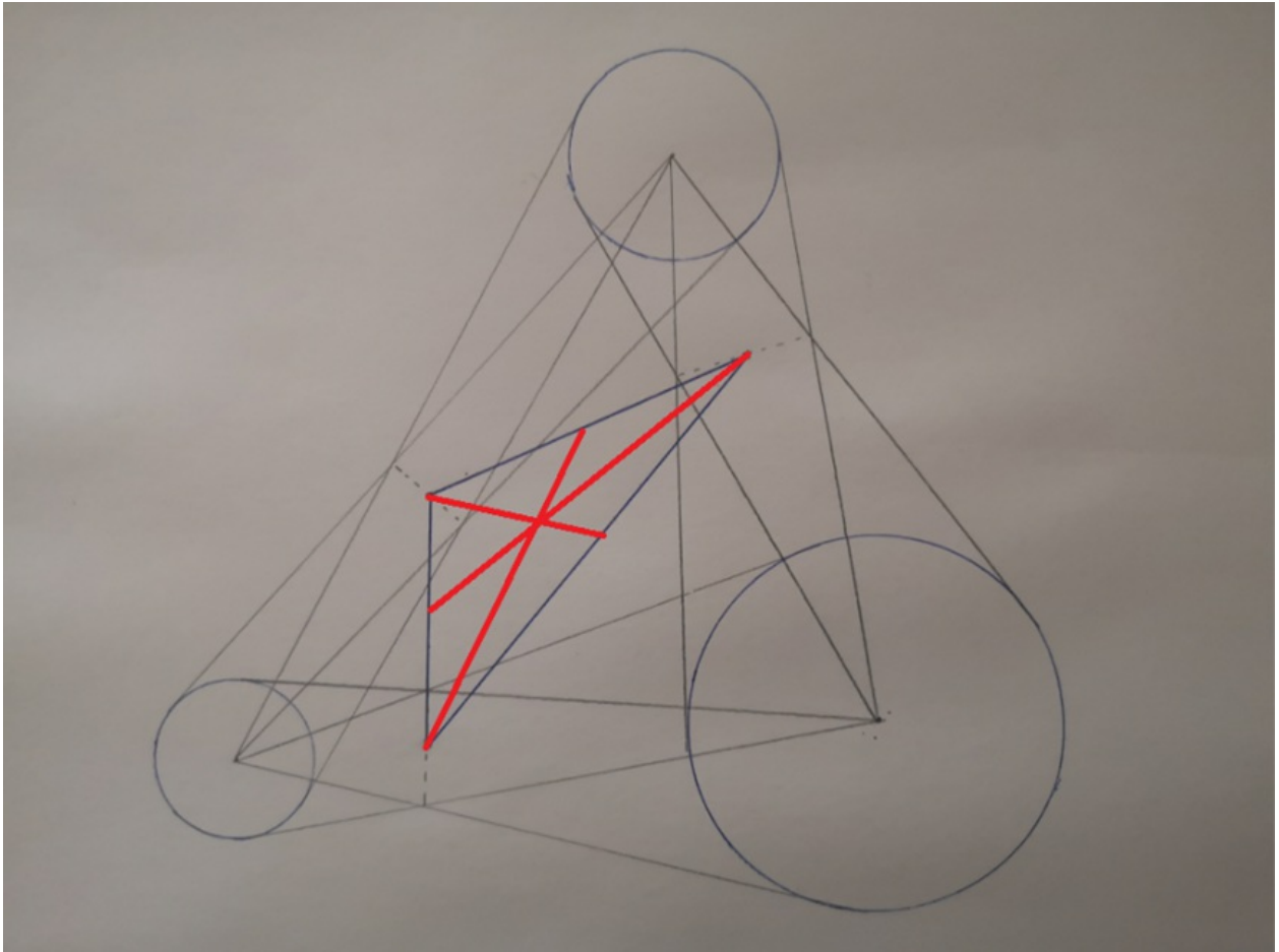
Fig. 2. First centroid
