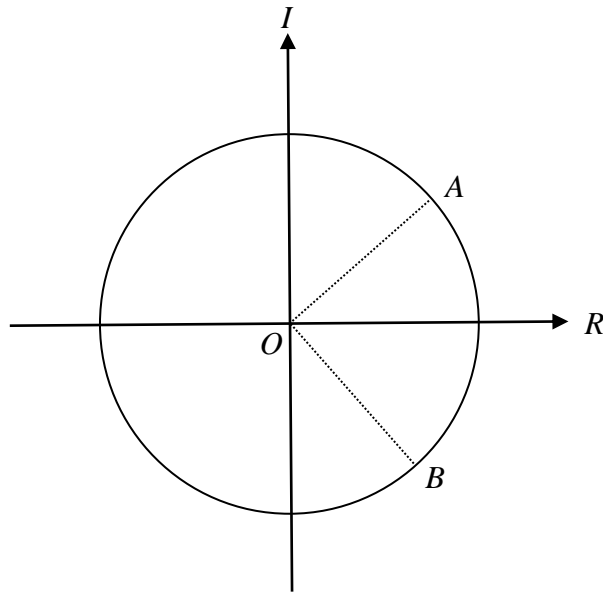
Figure 1. The complex time plane.
