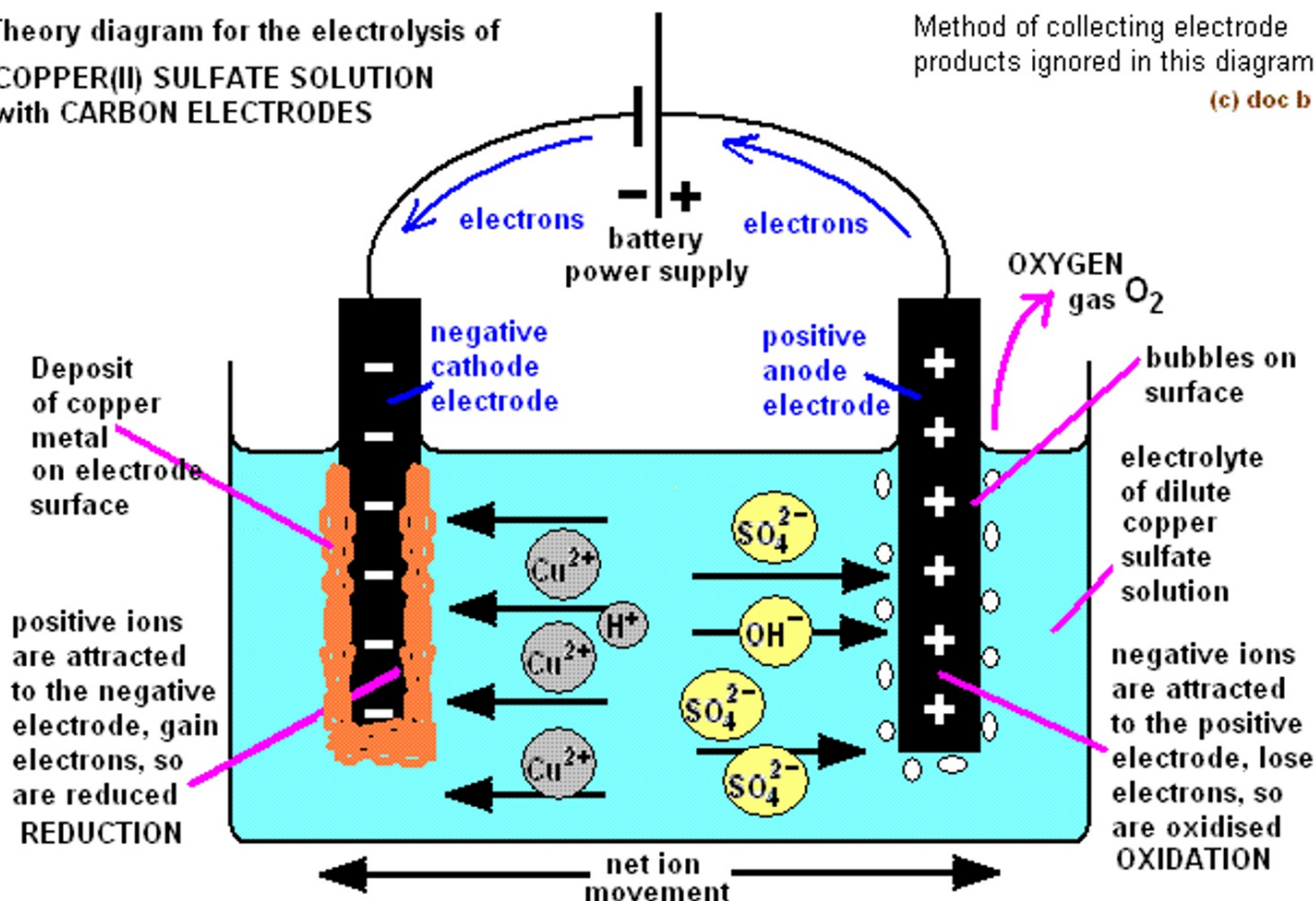
Figure 1. Diagram for the electrolysis of \text{Cu}^{2+} (Source: copied from Doc Brown's Chemistry, https://www.docbrown.info/page01/ExIndChem/electrochemistry04.htm ).
