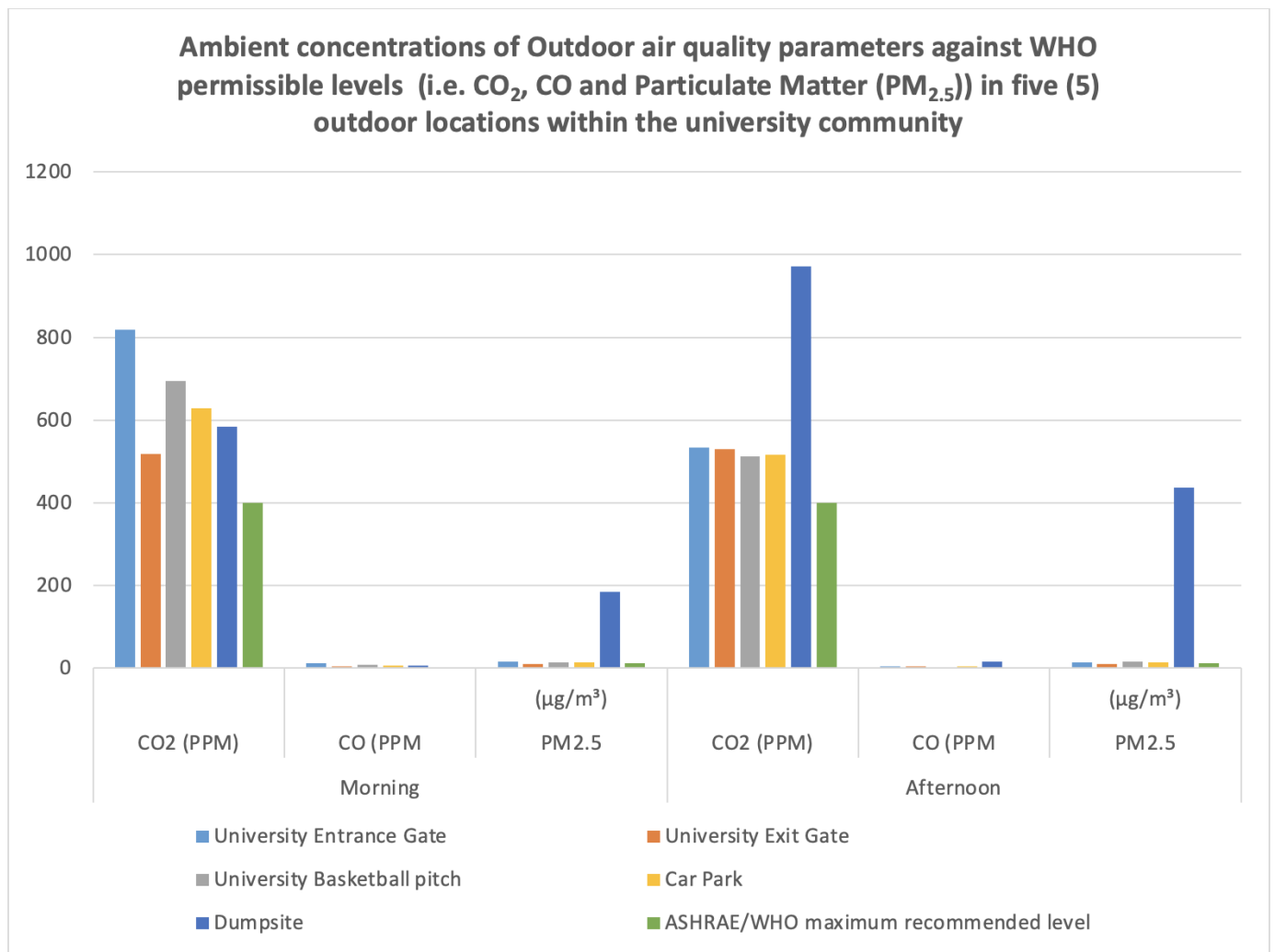
Figure 5. Ambient concentrations of outdoor air quality parameters against ASHRAE/WHO permissible levels (i.e. CO 2 , CO and Particulate Matter (PM 2.5 )) in five (5) locations within the university community
