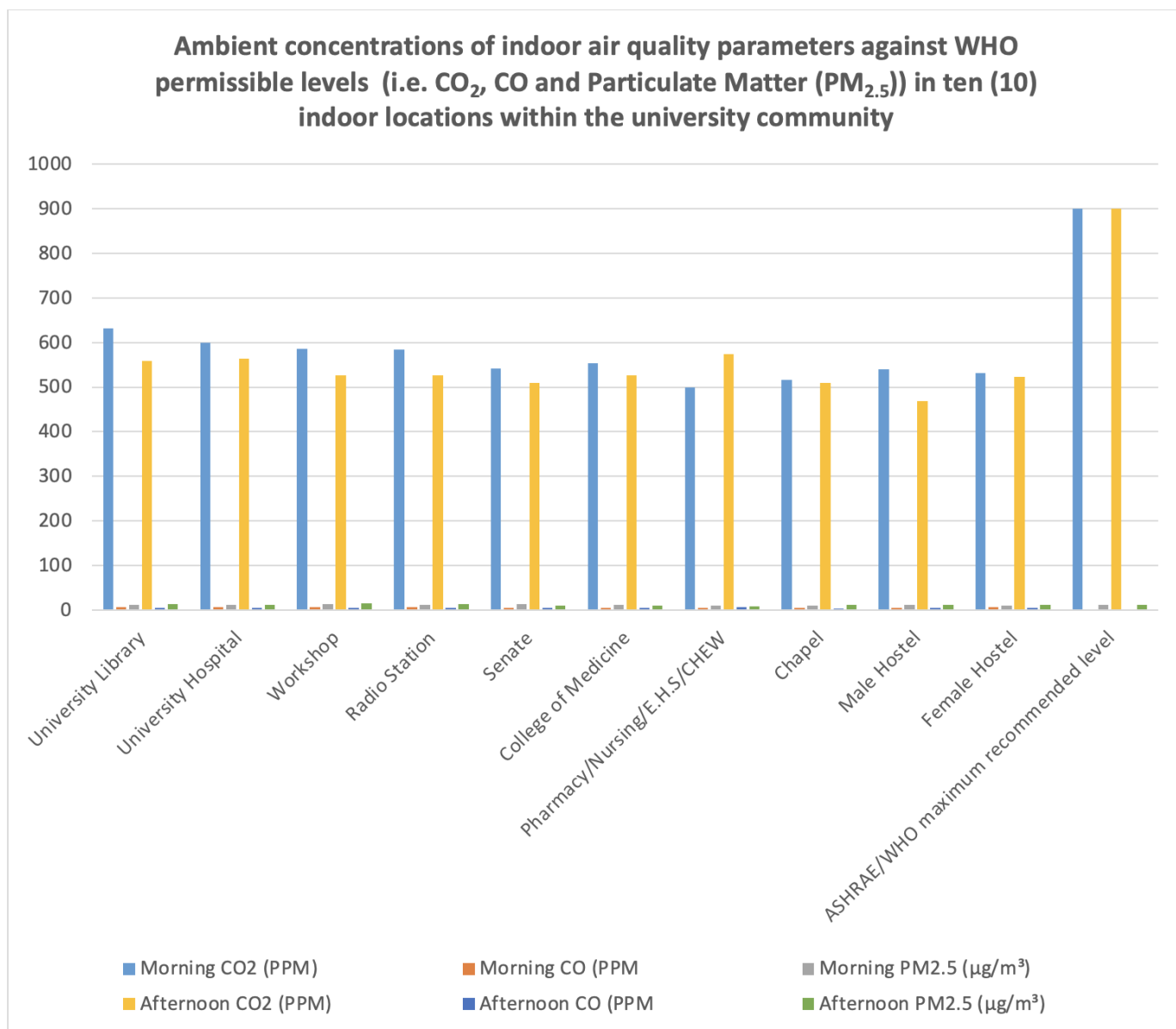
Figure 4. Ambient concentrations of indoor air quality parameters against ASHRAE/WHO permissible levels (i.e. CO 2 , CO and Particulate Matter (PM 2.5 )) in ten (10) locations within the university community
