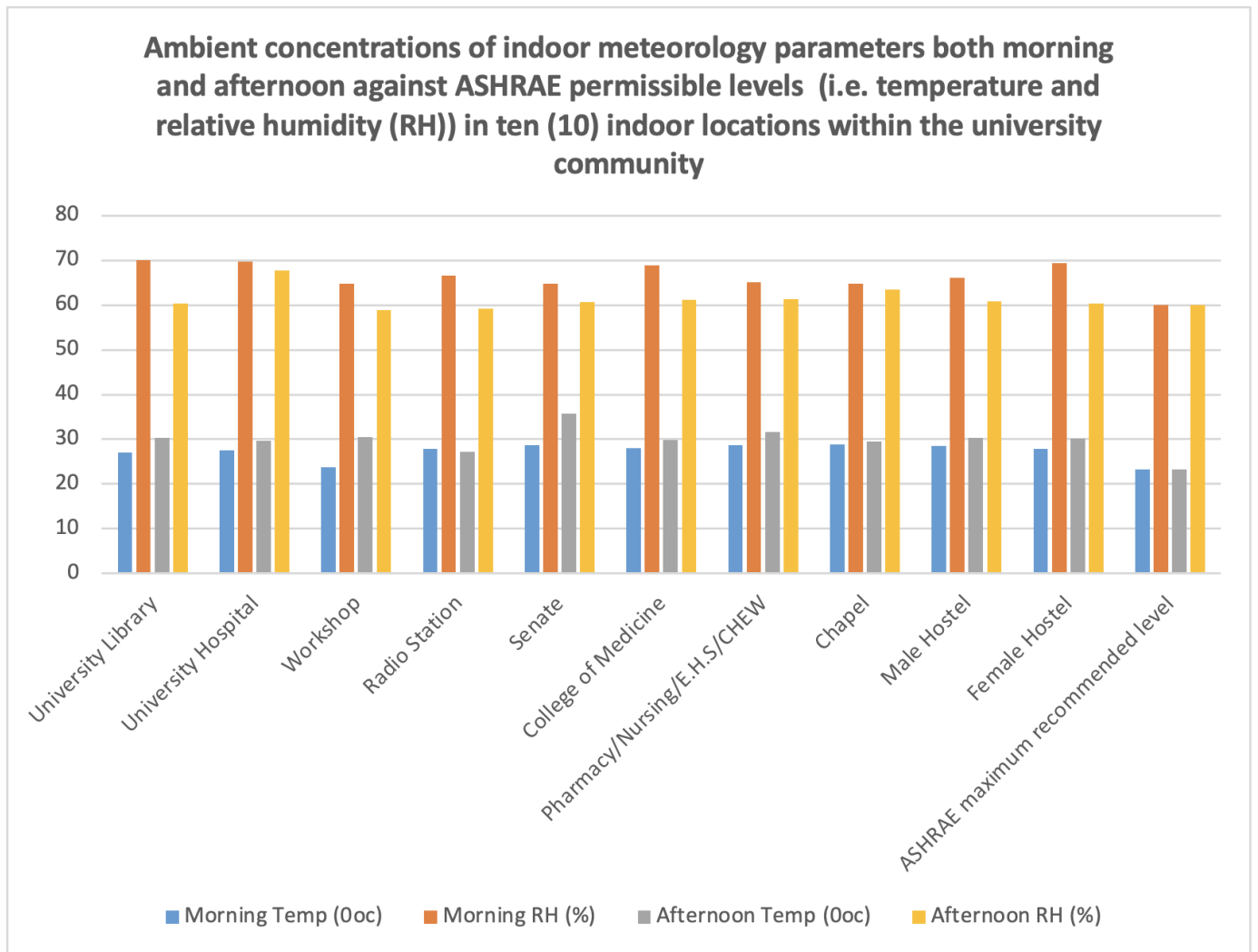
Figure 2. Morning and afternoon indoor meteorology (i.e. temperature and relative humidity (RH)) in ten (10) locations within the university community against ASHRAE permissible levels
