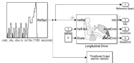
Fig. 10 Driver Input
