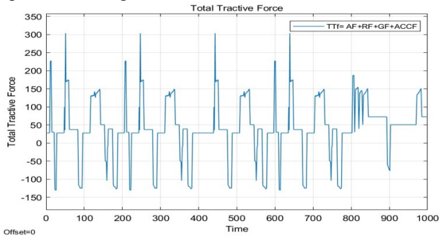
Fig. 19 Total Tractive Force
