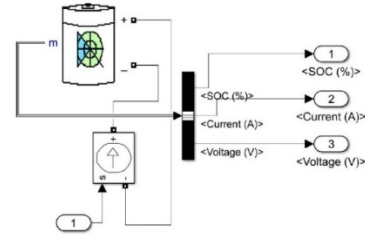
Fig. 11 Battery Subsystem
