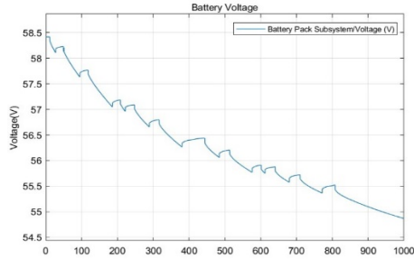
Fig. 23 Battery Voltage
