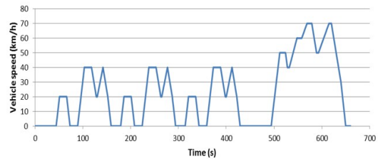
Fig.5 The 10-15 mode Japanese cycle
