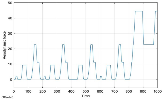
Fig. 16 Aerodynamic Force
