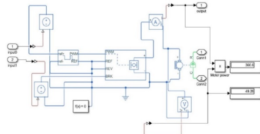
Fig. 12 Motor Circuit
