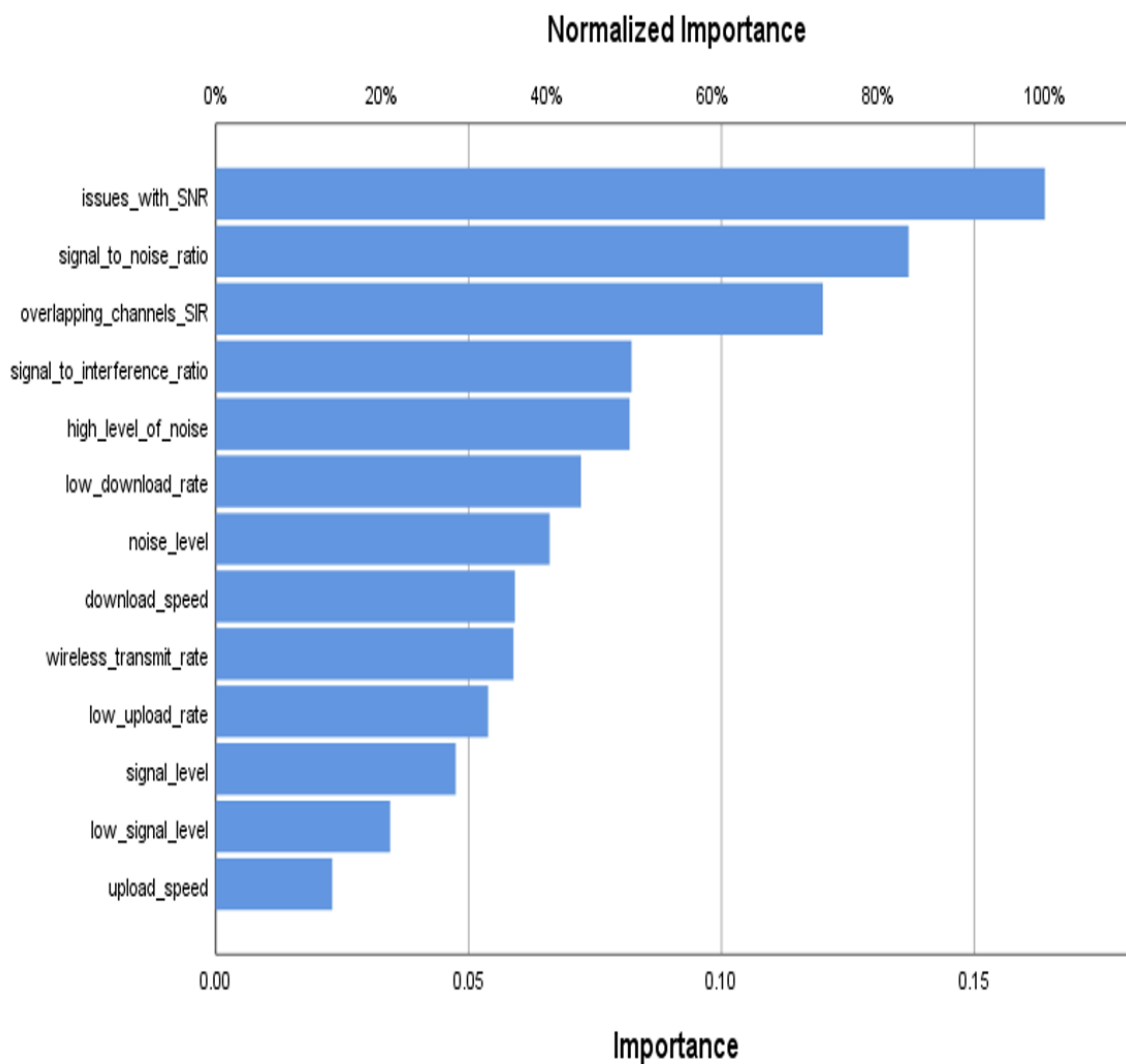
Fig. 9. Importance of Normalized for experimental test No. 1
