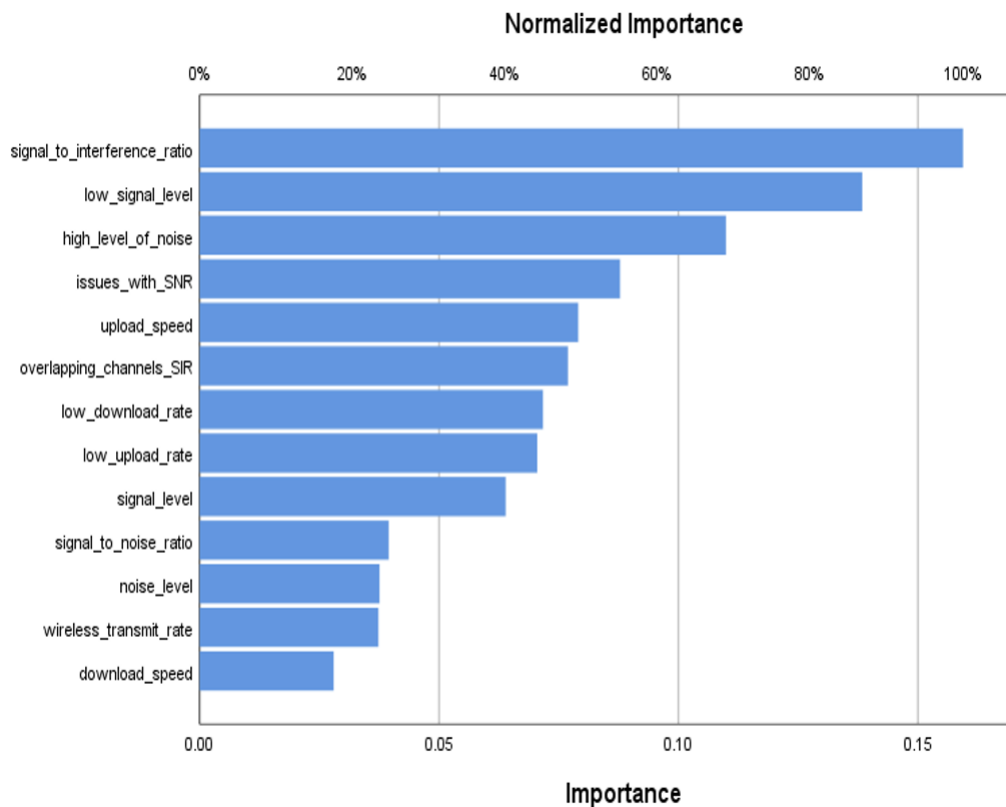
Fig. 10. Importance of Normalization for experimental test No. 2
