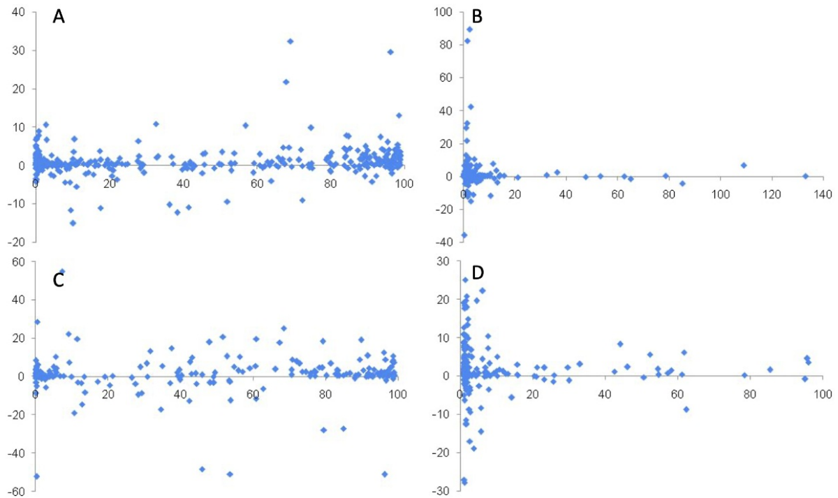
Figure 5. Correlations between the standing proportion of the new variant and the change in slope of the incidence curve (left panel) and between the proportionate increase in the new variant and the change in slope of the incidence curve (right panel). Panels A and B represent data for waves associated with the delta variant, while panels C and D represent data for waves associated with the omicron variant. The coefficient of determination ( r^2 ) for all four correlations was less than 10^{-4} .
