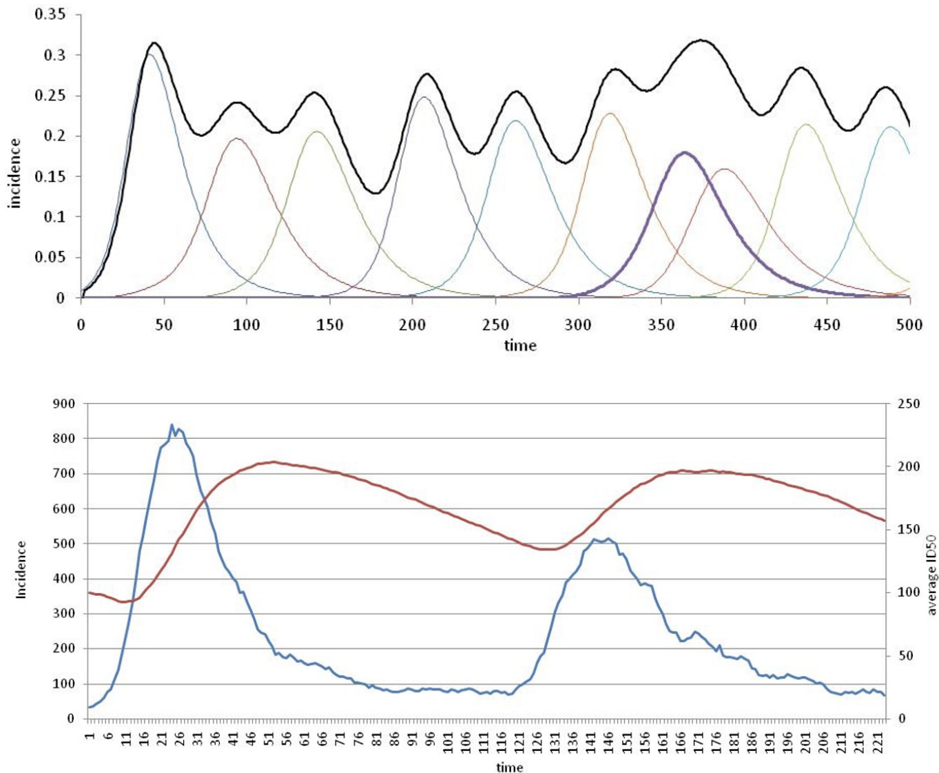
Figure 3. Example patterns observed in simulations using the two contrasting models. (a) SIR model incorporating the generation of novel immune-evading random mutations. The black line represents the total incidence, and the colored lines represent the incidence by successive variants. It is noteworthy that most new variants invade near the peaks of prior variants since the probability of mutation is highest during that time. (b) Result of the Watve et al. (2021) model, demonstrating waves separated by a significant period of low incidence resembling an apparently endemic state. The blue line represents the incidence curve, and the red line represents the mean population immunity. In this model, waves are observed even in the absence of a new variant.
