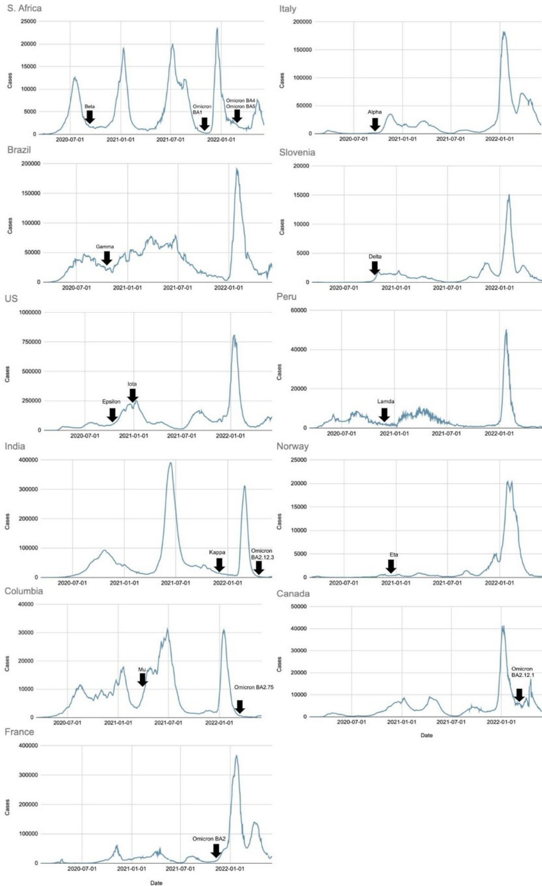
Figure 6. The countries and time of origin for the 16 variants and sub-variants being monitored. The origin of a new variant is indicated by an arrow along the incidence curve. It is noteworthy that the majority of variants were first
