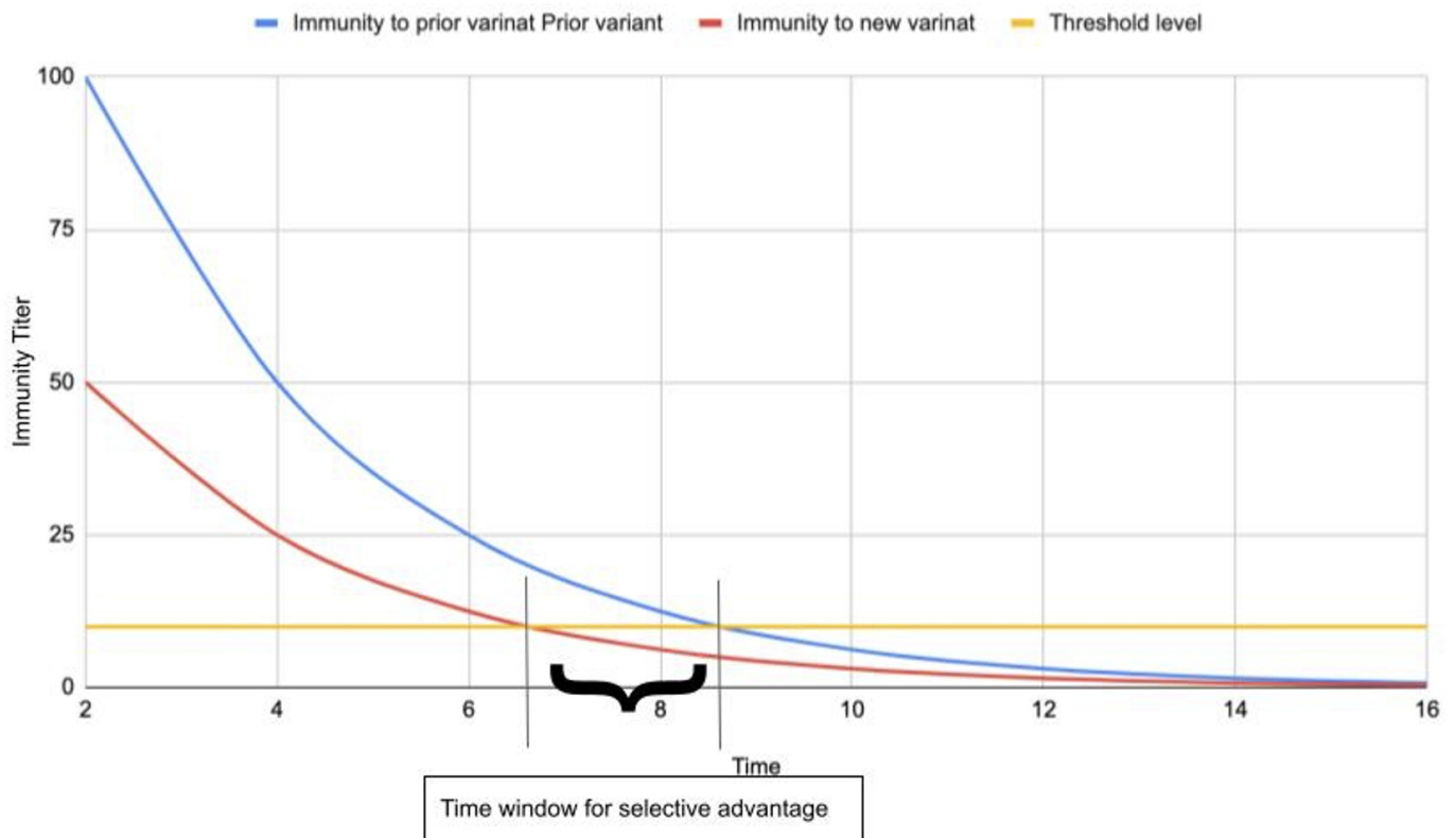
Figure 1. Dynamics of immunity and selection of the new variant: The partially immune variant is expected to have a lower immunity titer. Assuming the rate of immunity loss is the same, the new variant can cross the minimum immunity threshold before the old variant does, creating a window for selection. Beyond this window, there is no clear advantage for the new variant.
