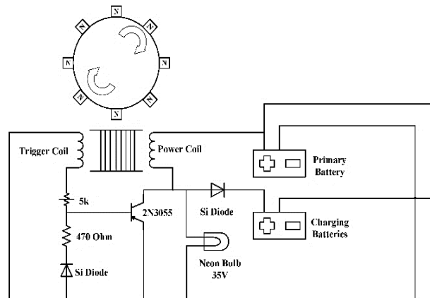
Figure 7: Operational circuit for Bedini SSG
