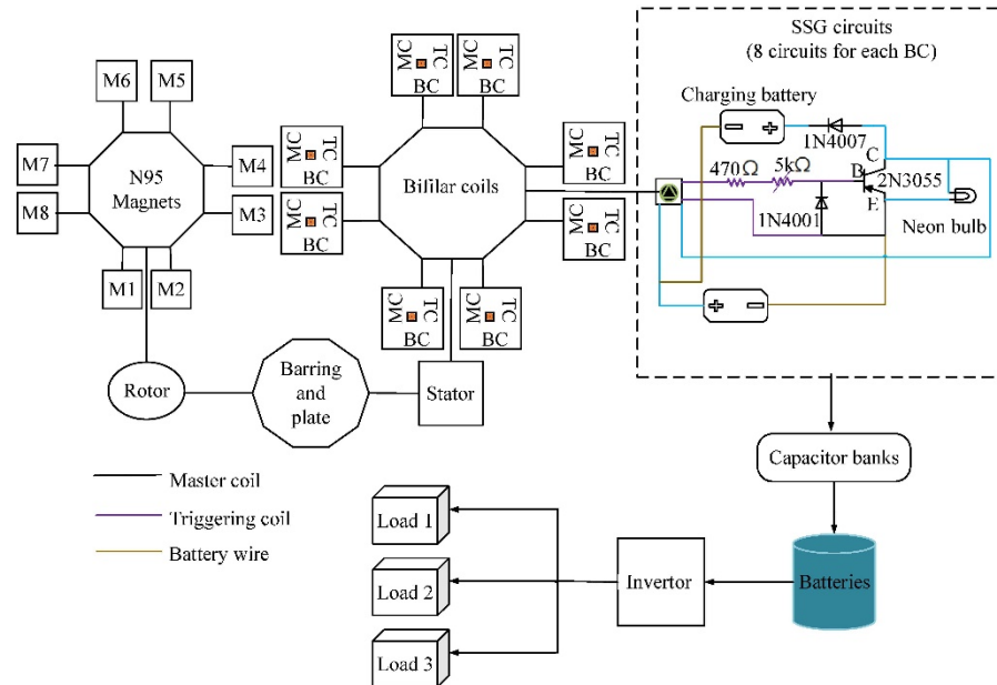
Figure 8: Proposed MFEG's schematic
