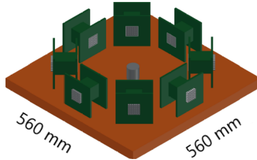
Figure 5: Stator design
