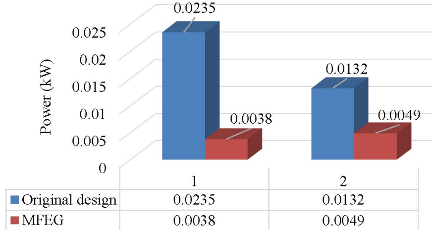
Figure 10: Comparison between original design and MFEG
