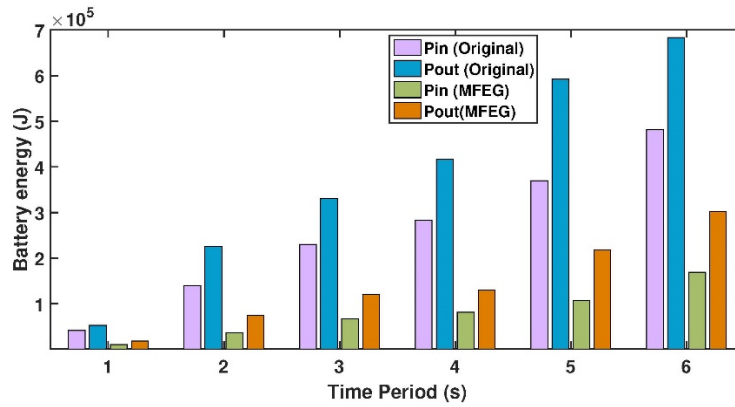
Figure 12: Battery's power
