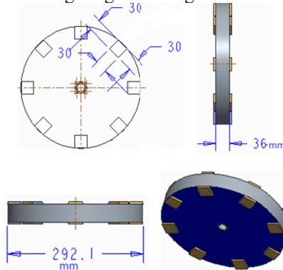
Figure 3: Rotor design
