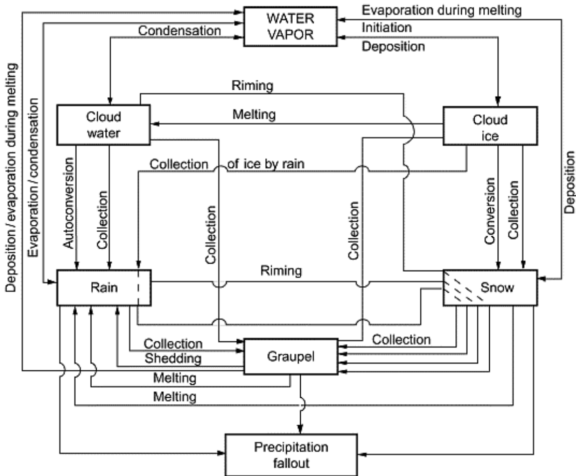
Figure 2: Cloud particle lifecycle (Robert A Houze, 2014) (8)
