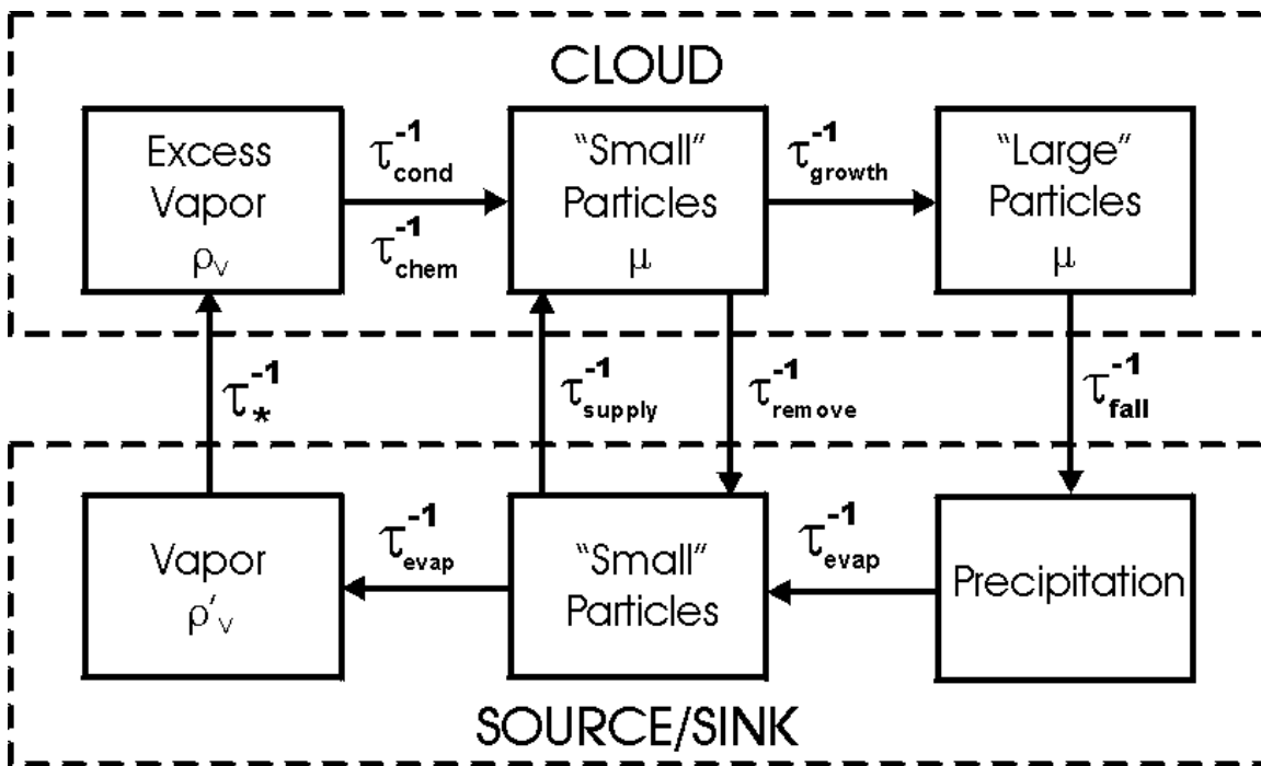
Figure 1. The microphysics of cloud formation (R.Schmunk, 2019) (11)
