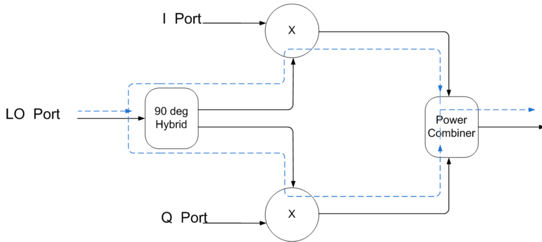
Figure 3. Leakage path in Mixer
