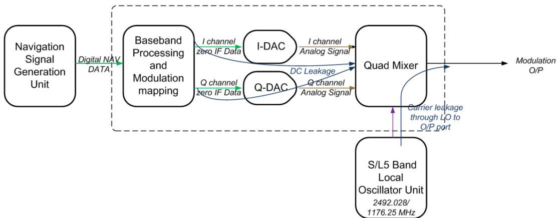
Figure 4. Leakage path in modulator
