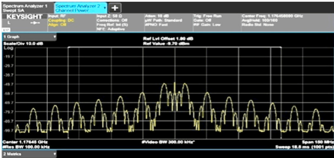
Figure 5. Frequency Spectrum with Carrier Leakage
