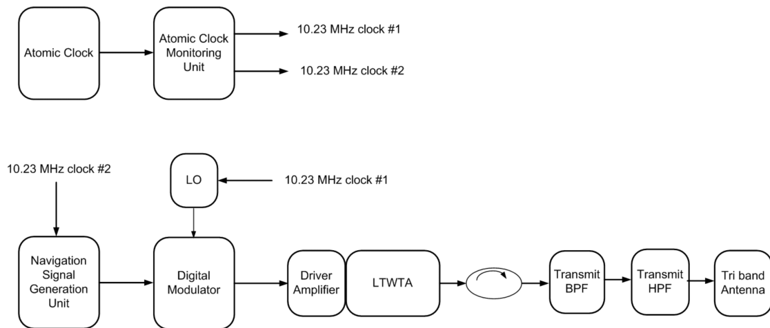
Figure 1. NAVIC Navigation Payload architecture (NVS-01)
