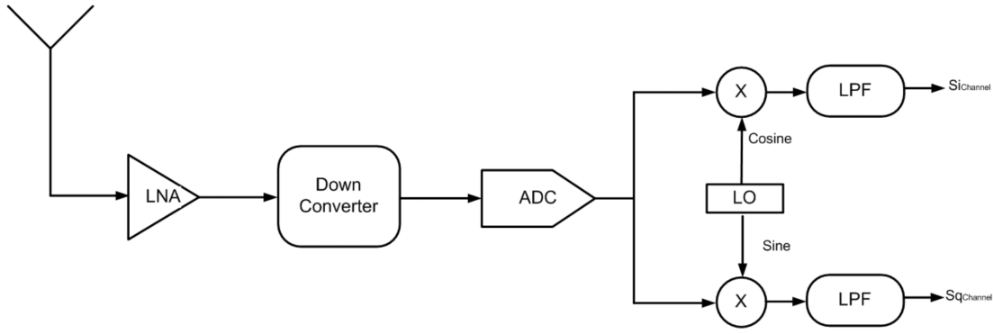
Figure 7. Block Diagram of GNSS Receiver
