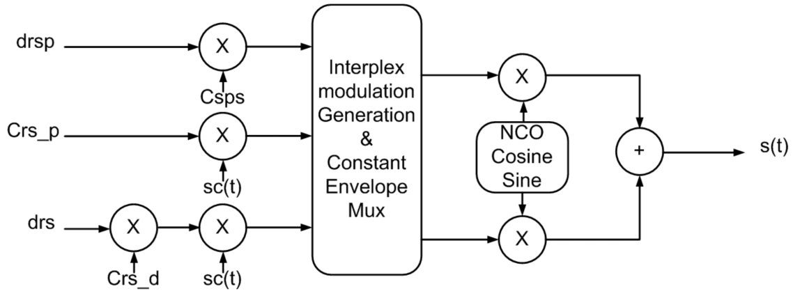
Figure 2. Block schematic for composite signal generation
