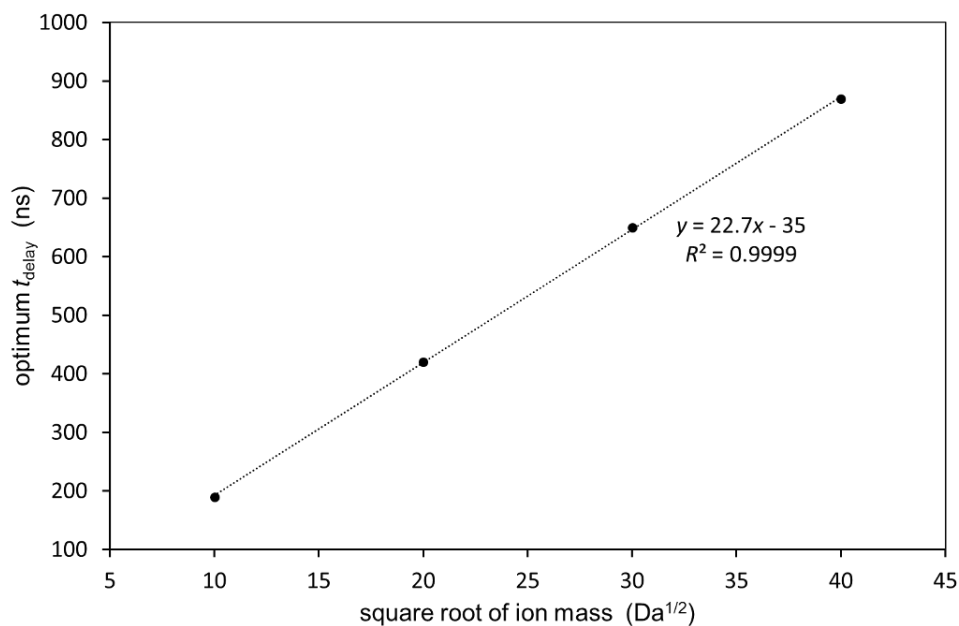
Figure 11. Linear correlation plots between square root of ion mass and the optimum t_{\text{delay}} that maximizes R_{\text{TOF}} at the fixed value of V_{\text{PEDA}} = 400 V.
