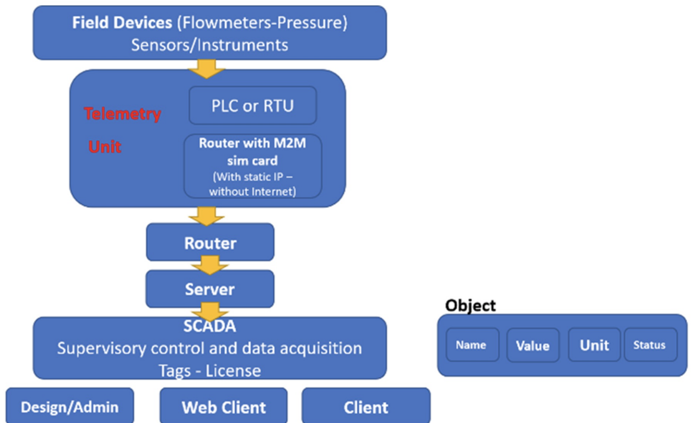
Fig. 3. Flow Chart from Field Devices to SCADA application.
