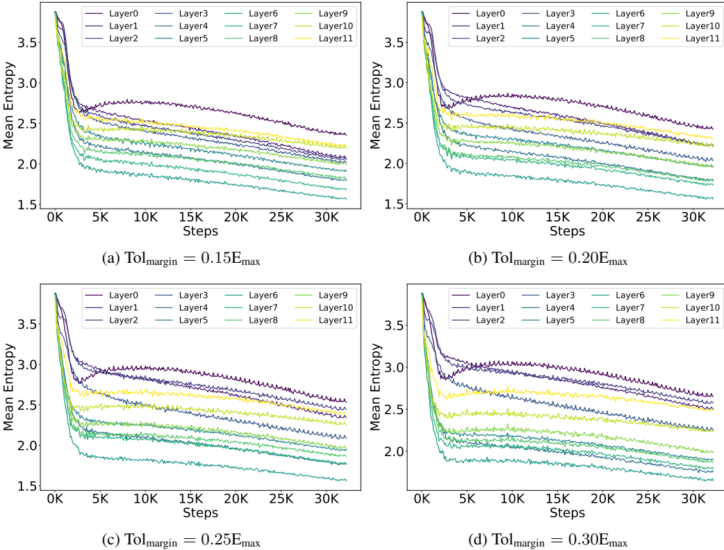
Figure 19: Layerwise entropy dynamics when entropy regularization is employed with increasing threshold margin, defined as \text{ToI}_{\text{margin}} = \gamma E_{\text{max}} (see Algorithm1, line #3). At higher \gamma , the mean entropy of the early layers increases.
