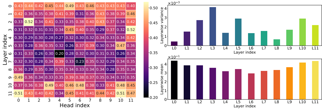
Figure 10: Analysis of learned threshold weights ( reg_threshold_weights , see Eq. 4.3) in entropy regularization for softmax-only GPT-2 model: (a) Attention heads adaptively learn non-uniform threshold weights across different heads, setting individualized thresholds for entropy regularization; (b) The non-uniform means and non-zero variances across layers highlight the necessity and effectiveness of headwise learnable thresholds in adapting regularization strength.
