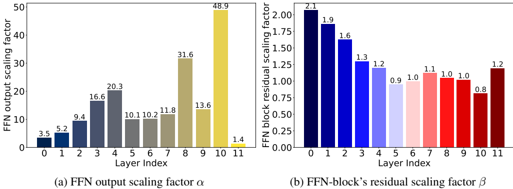
Figure 11: Learned scaling factors \alpha and \beta in Eq. 6 across different layers in the Softmax-only GPT-2 model ( L=12, H=12, d=768 ). The values were plotted after full model training to observe the modulation of FFN outputs and residual connections in each layer.
