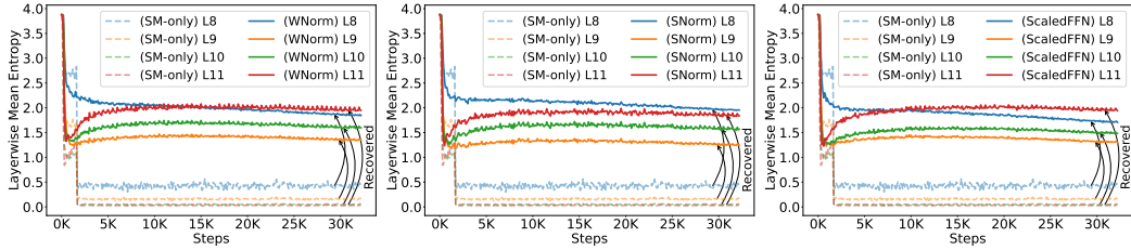
(a) Weight normalization in FFN (b) Spectral normalization in FFN (c) Learnable scaling of FFN outputs Figure 7: Mitigating entropy collapse in the deeper layers of a softmax-only GPT-2 model by employing weight or spectral normalization in FFN, or by appropriately scaling FFN block outputs.
