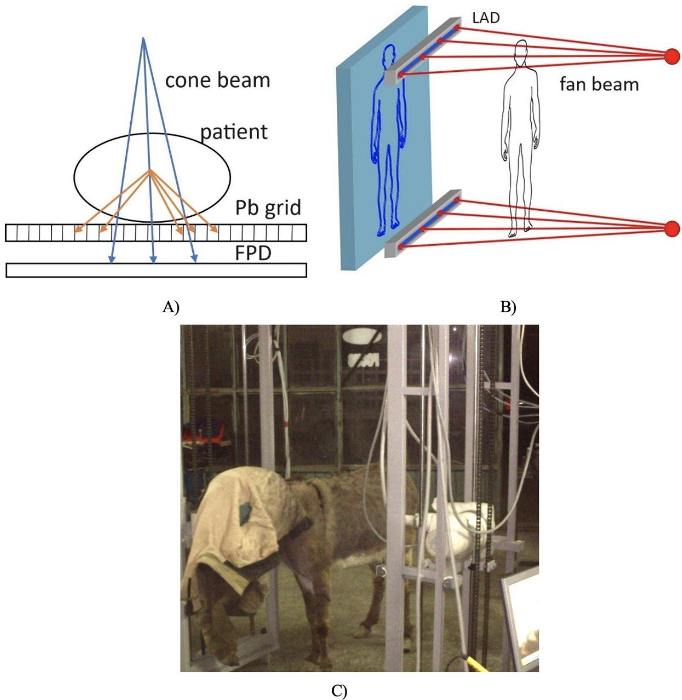
Figure 1. A) FPD and anti-scatter Pb grid which attenuates scattered photons from cone beam and let direct photons to form the image B) LAD with fan beam C) Four years old female donkey.
