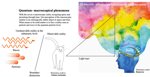
Figure 3. Illustrates the quantum-holographic-informational system
