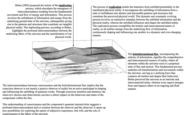
Figure 1. Illustrates the holoinformational flux. Illustration credits to (Oberleithner, 2012)
