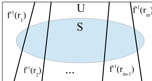
Figure 1: Subset S expressed as union over r \in f(U) of disjoint intersections f^{-1}(r) \cap S
