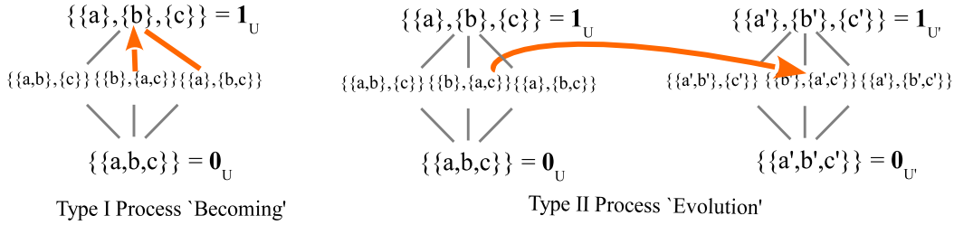
Figure 4: Skeletal representation of Type I and Type II processes using partition lattices
